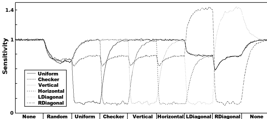
Figure 5: The sensitivity graph produced by the illustrative neural network. In addition to the environments seen in figure 4, this graph shows the networks response to the left diagonal and right diagonal environments.
