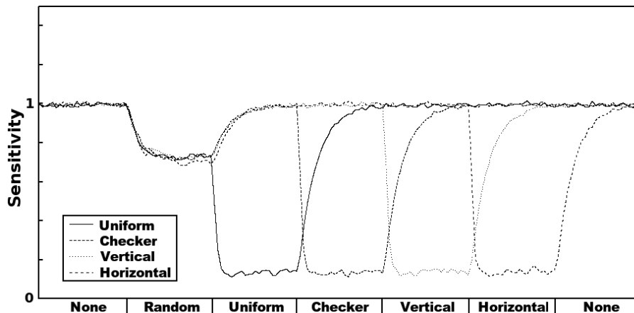
Figure 4: The sensitivity graph produced by the illustrative neural network given in [7]. This shows how sensitivity to the uniform, checkerboard, vertical bar and horizontal bar environments vary as the network adapts to each environment during the time course of the simulation.
