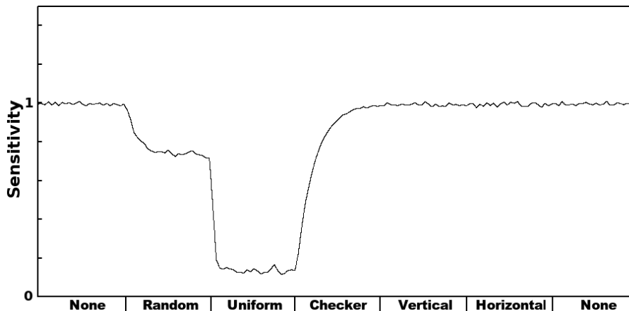
Figure 3: The sensitivity graph produced by the illustrative neural network given in [7]. This shows how sensitivity to the uniform environment varies during the time course of the simulation. A sensitivity close to zero indicates that the environment is known and that the output of the network is small. Conversely, a sensitivity close to one indicates that the environment is novel and that the output is close to the sum of the intensities in the centre patch.
