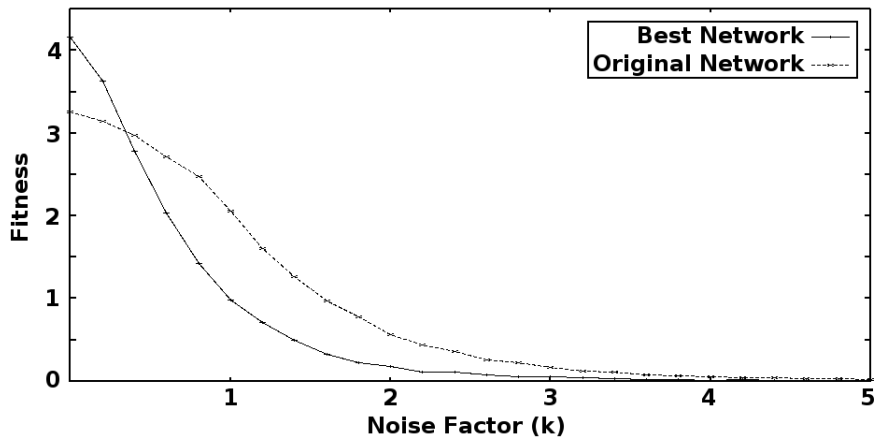
Figure 7: Fitness of the best evolved network as noise is applied to its inputs, with noise factor k varied from 0.0 to 5.0
