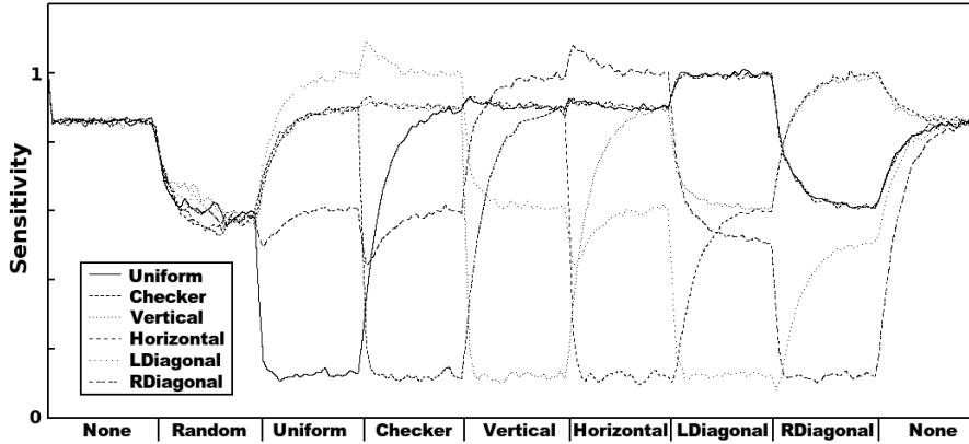
Figure 6: The sensitivity graph produced by the best network found by NEAT.
