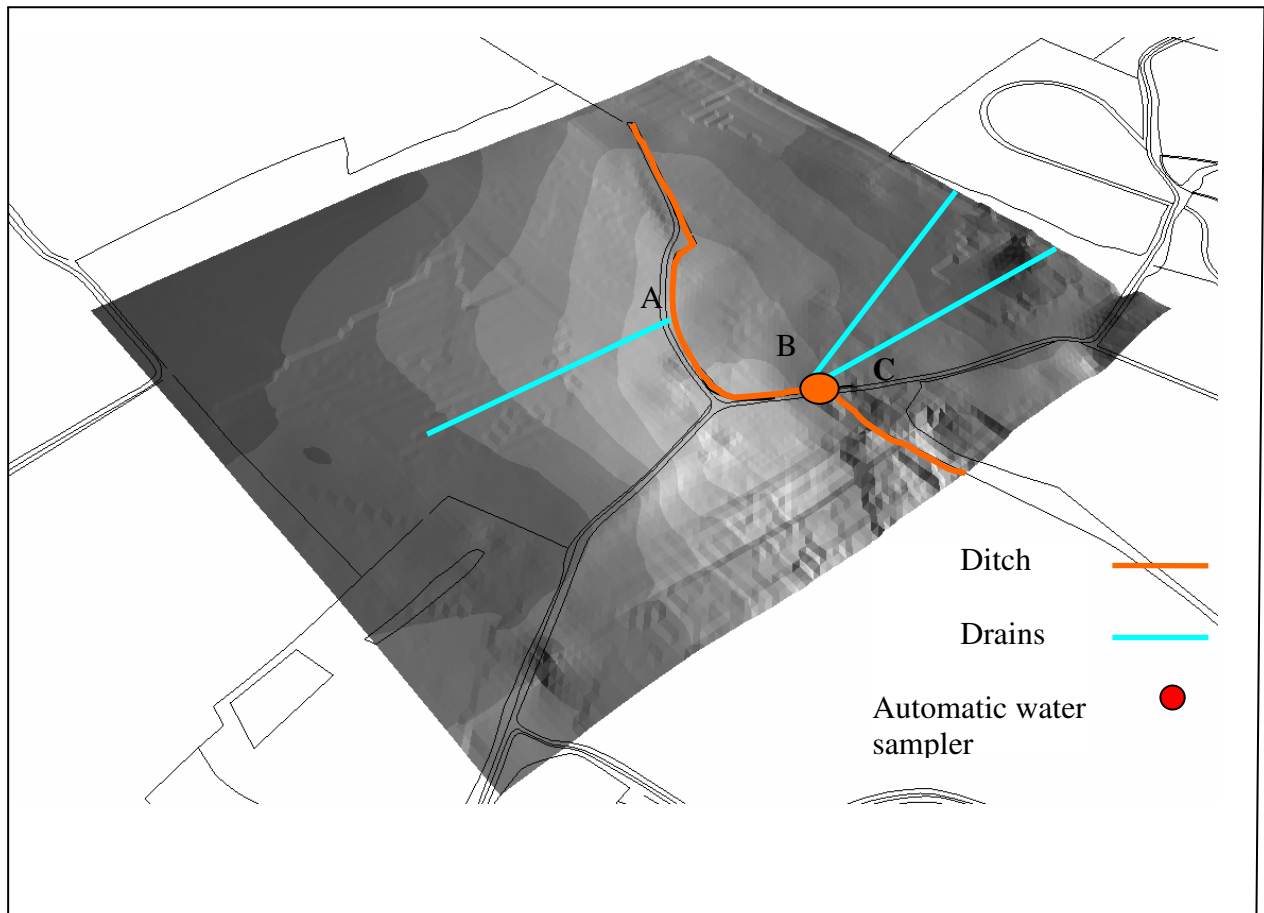
Figure 4 DTM of Field B with individual sampling points identified A,B, and C
